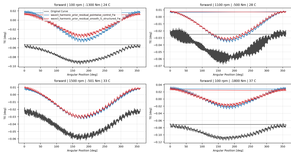
Forward Wave 3 Harmonic Prior Residual Registry Overlay TE Curve Verification Pipeline comparison
