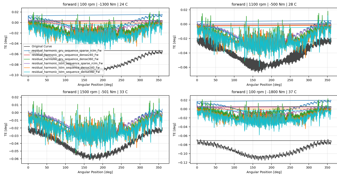
Forward Wave 2.3 Residual Harmonic Temporal Overlay TE Curve Verification Pipeline comparison
