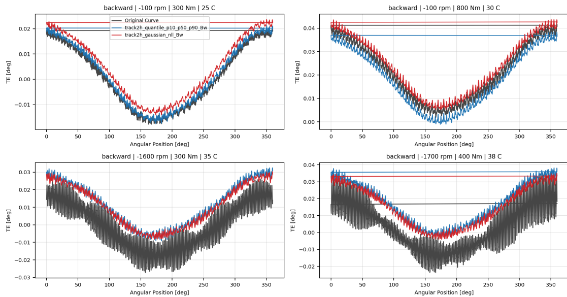
Backward Wave 4.2 Quantile Probabilistic Overlay TE Curve Verification Pipeline comparison
