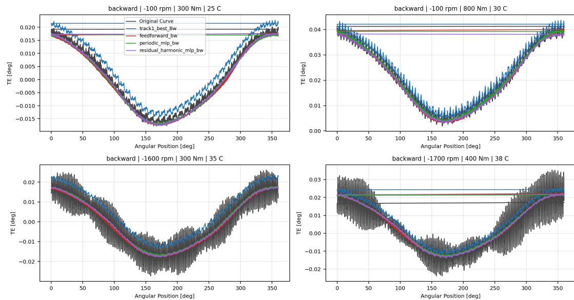
Backward RCIM Model-Bank Reproduction And Screened Wave 1 Overlay TE Curve Verification Pipeline comparison
