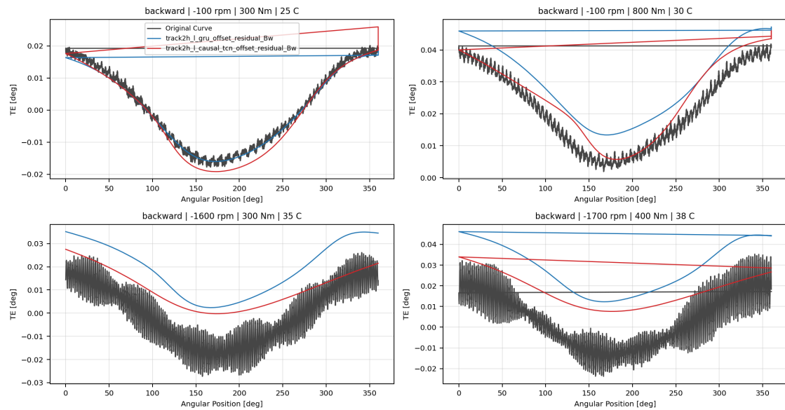
Backward Wave 4.4 Latent State Hysteresis Overlay TE Curve Verification Pipeline comparison
