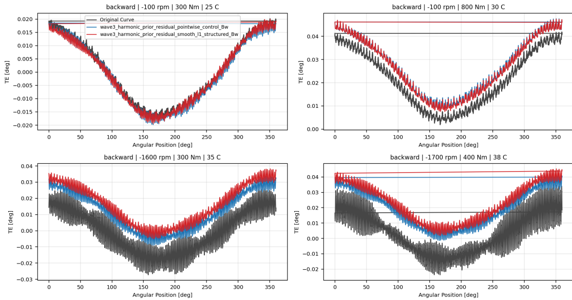
Backward Wave 3 Harmonic Prior Residual Registry Overlay TE Curve Verification Pipeline comparison
