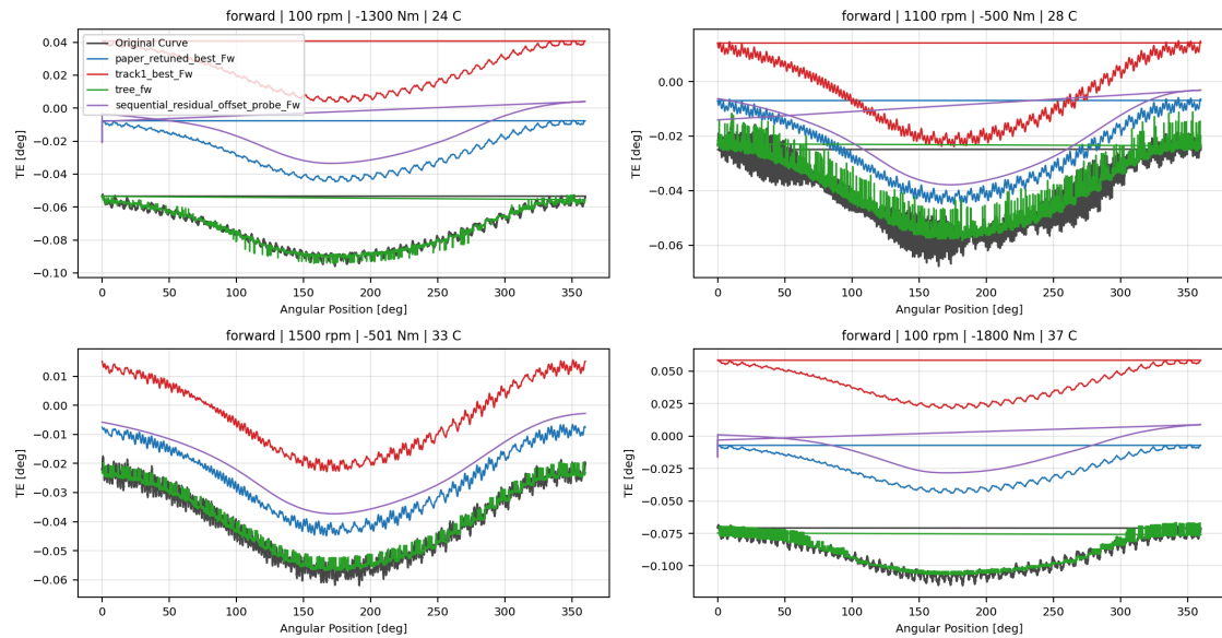
Forward Reference Tree And Wave 3.1 Overlay TE Curve Verification Pipeline comparison
