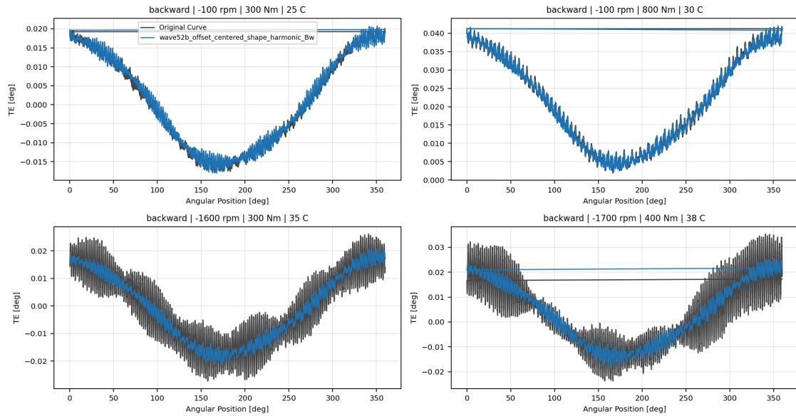
Backward Wave52b Offset Harmonic Guided Registry Overlay TE Curve Verification Pipeline comparison
