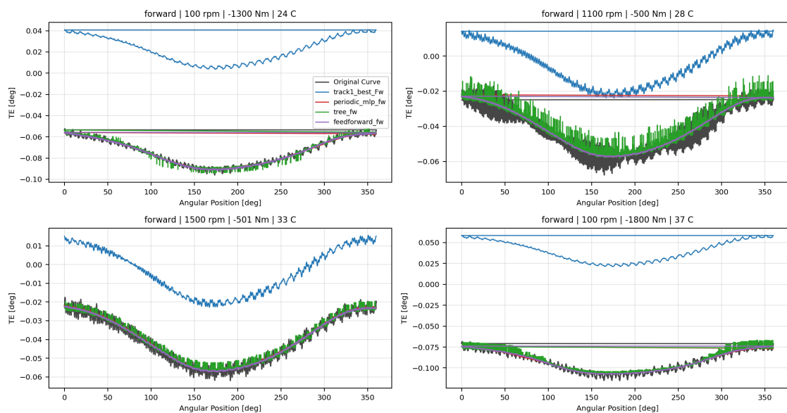
Forward RCIM Model-Bank Reproduction And Screened Wave 1 Overlay TE Curve Verification Pipeline comparison
