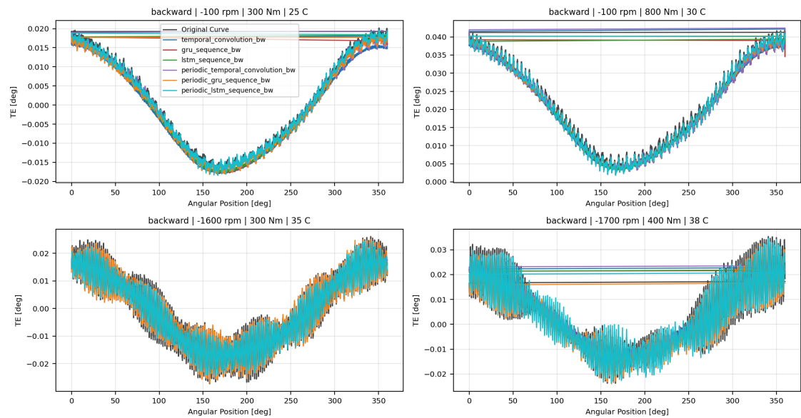
Backward Wave 2.1 Temporal Model Overlay TE Curve Verification Pipeline comparison
