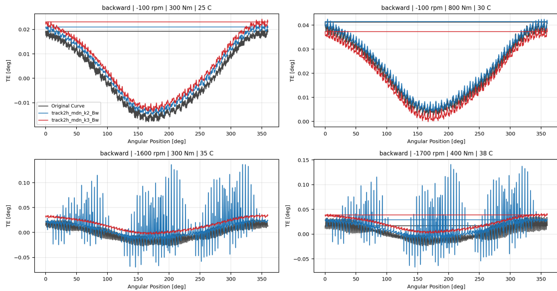
Backward Wave 4.3 Mixture Density Overlay TE Curve Verification Pipeline comparison
