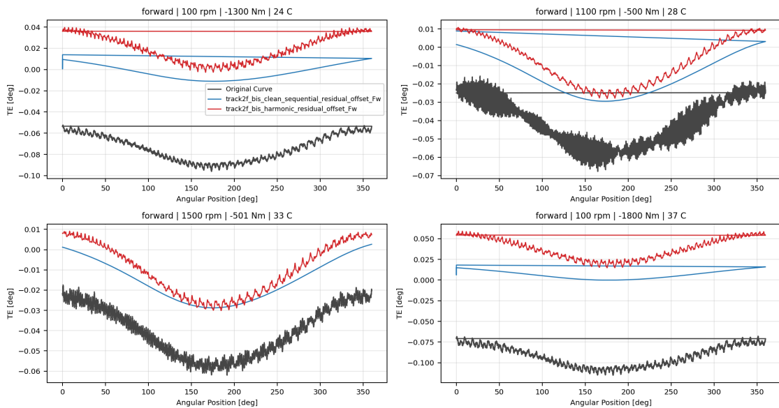
Forward Wave 3.2 Harmonic-Offset Probe Overlay TE Curve Verification Pipeline comparison
