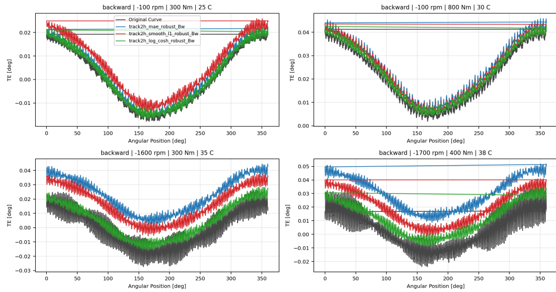
Backward Wave 4.1 Robust-Loss Overlay TE Curve Verification Pipeline comparison
