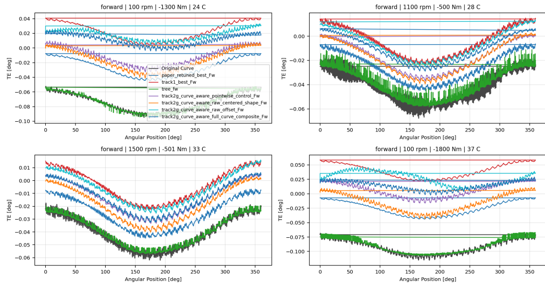
Forward Reference Tree And Wave 3.3 Overlay TE Curve Verification Pipeline comparison
