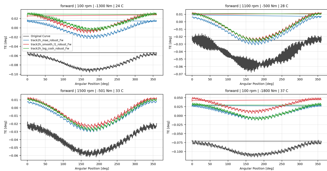
Forward Wave 4.1 Robust-Loss Overlay TE Curve Verification Pipeline comparison
