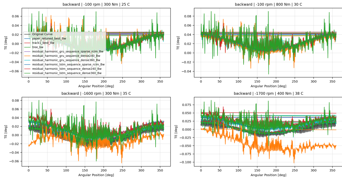
Backward Reference Tree And Wave 2.3 Overlay TE Curve Verification Pipeline comparison
