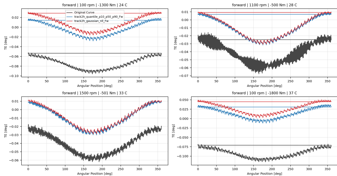
Forward Wave 4.2 Quantile Probabilistic Overlay TE Curve Verification Pipeline comparison
