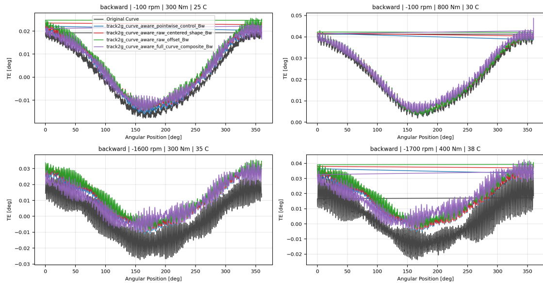
Backward Wave 3.3 Curve-Aware Training Overlay TE Curve Verification Pipeline comparison
