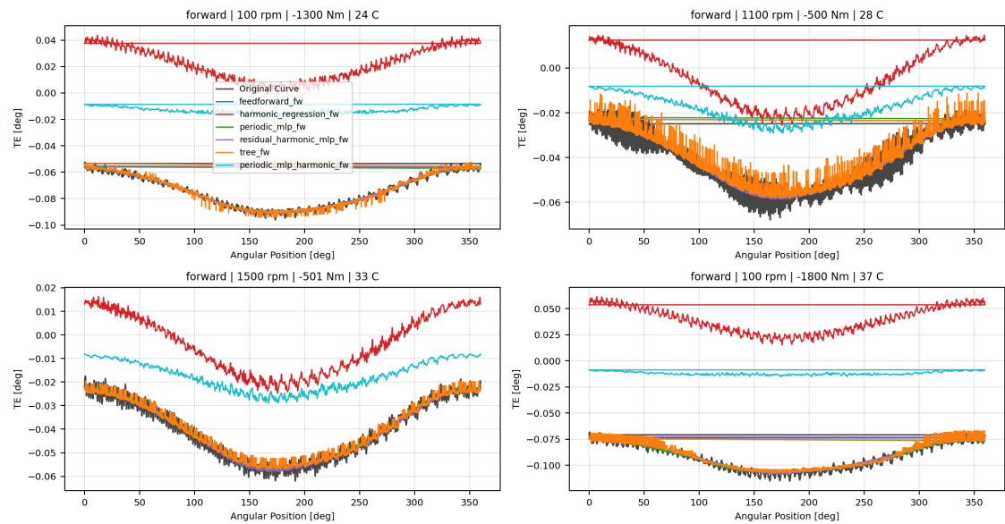
Forward Wave 1 Family Model Overlay TE Curve Verification Pipeline comparison
