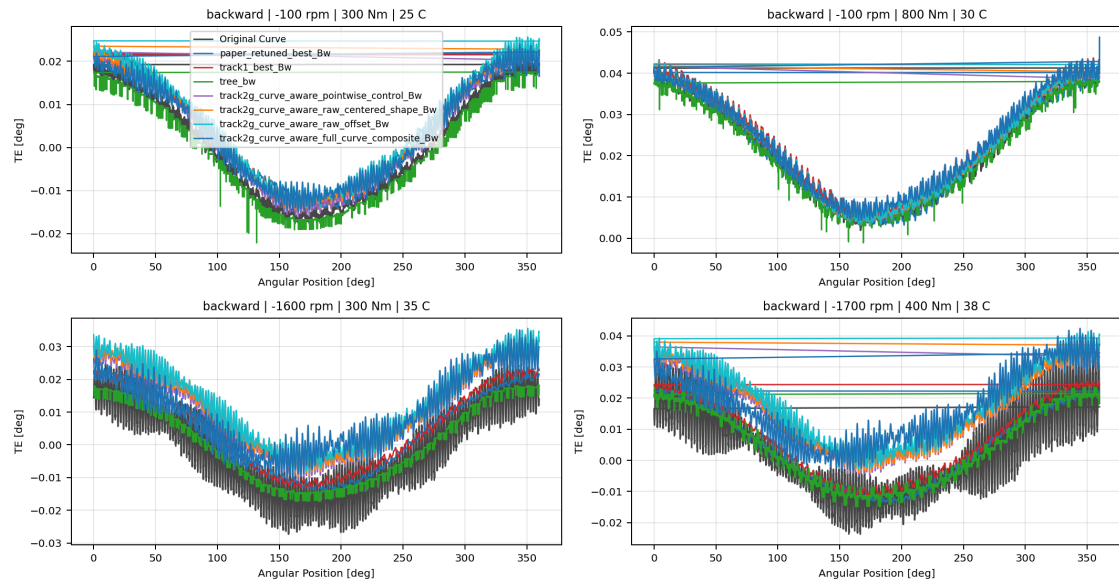
Backward Reference Tree And Wave 3.3 Overlay TE Curve Verification Pipeline comparison
