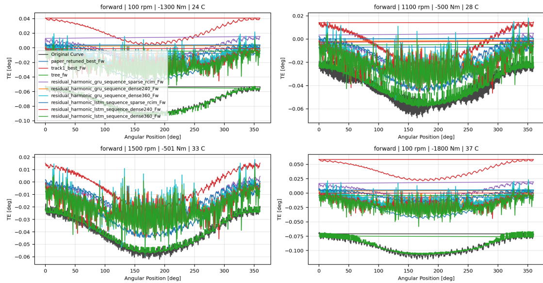
Forward Reference Tree And Wave 2.3 Overlay TE Curve Verification Pipeline comparison
