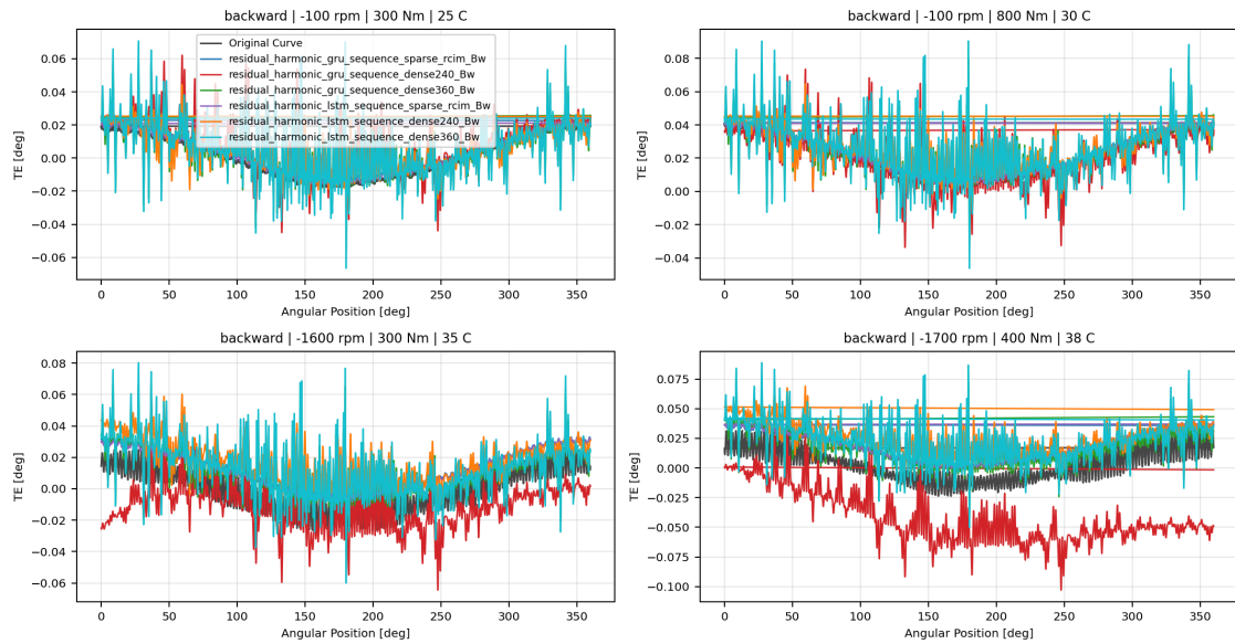
Backward Wave 2.3 Residual Harmonic Temporal Overlay TE Curve Verification Pipeline comparison
