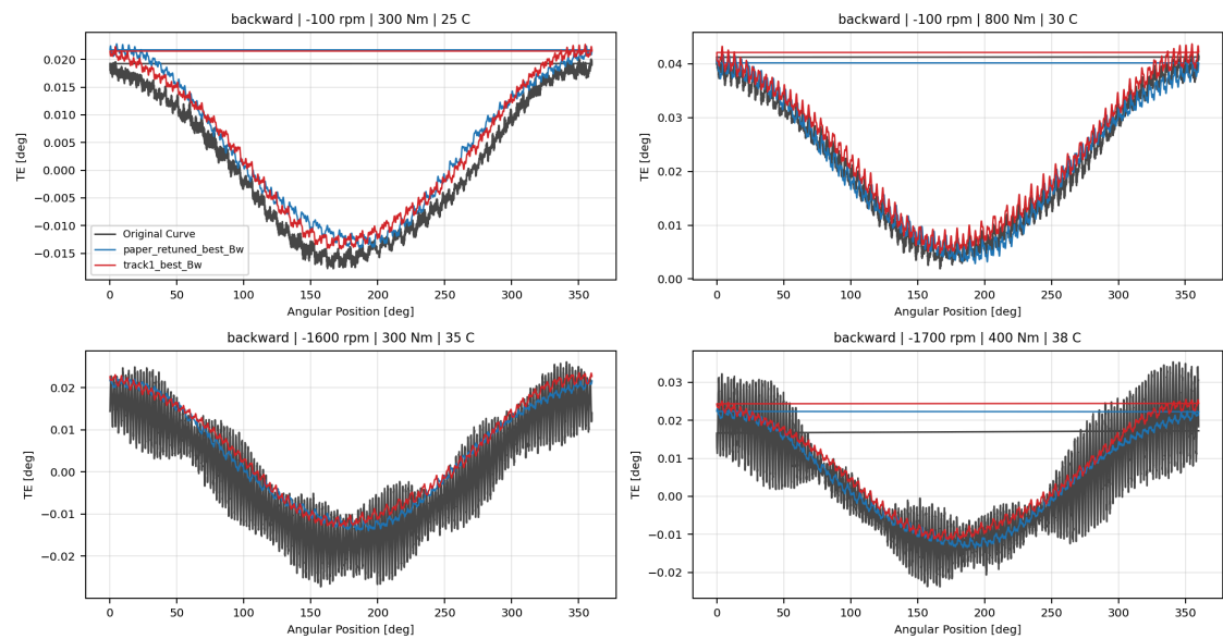
Backward Reference Model Overlay TE Curve Verification Pipeline comparison
