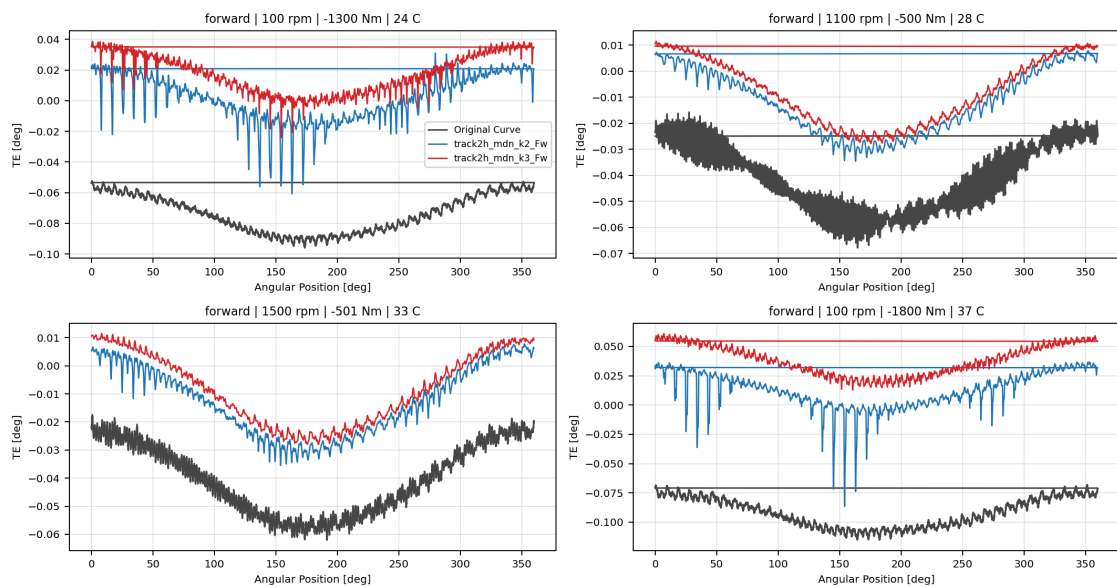
Forward Wave 4.3 Mixture Density Overlay TE Curve Verification Pipeline comparison
