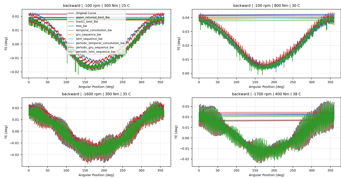
Backward Reference Tree And Wave 2.1 Overlay TE Curve Verification Pipeline comparison
