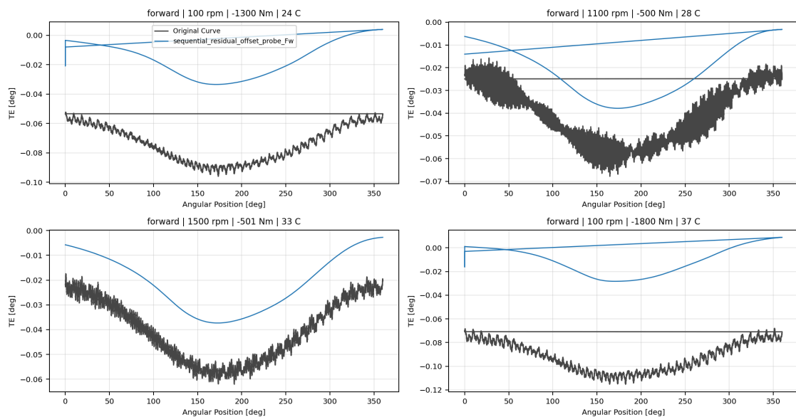
Forward Wave 3.1 Offset-Aware Probe Overlay TE Curve Verification Pipeline comparison
