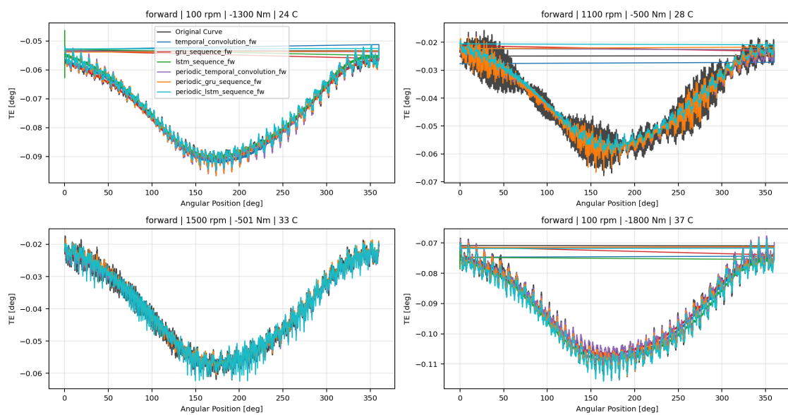
Forward Wave 2.1 Temporal Model Overlay TE Curve Verification Pipeline comparison
