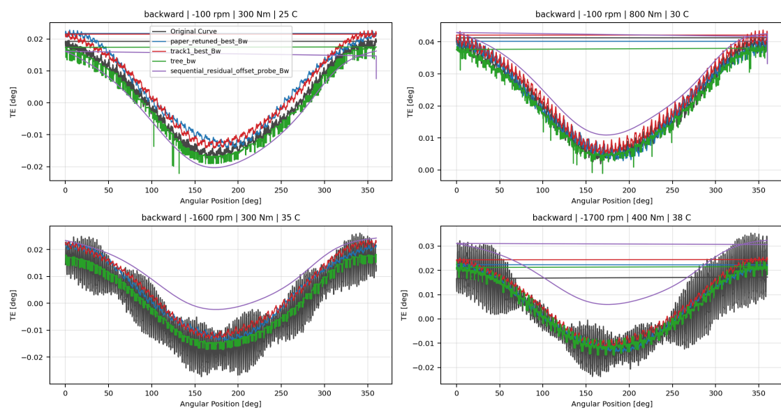
Backward Reference Tree And Wave 3.1 Overlay TE Curve Verification Pipeline comparison
